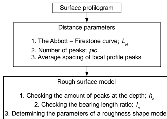
Fig. 6. Algorithm for building a rough surface model
