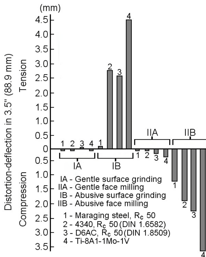
Fig. 13. Deformations of a sample subjected to grinding and milling [12]
