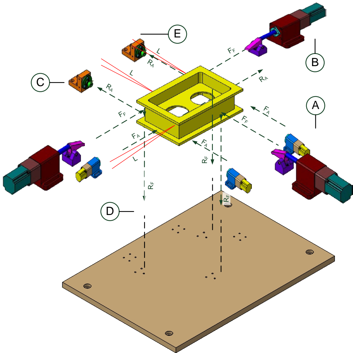
Fig. 2 Overview of a device with indications of important values; A – alignment actuators, B – fixing actuators, C – alignment locators with force sensors, D – fixing locators with force sensors, E – laser sensors of large displacements, F_A – forces exerted by alignment actuators, F_F – forces exerted by fixing locators, R_A – reaction forces on alignment locators, R_F – reaction forces on fixing locators, L – measured distances of a workpiece from actuator tips in the rest position.
